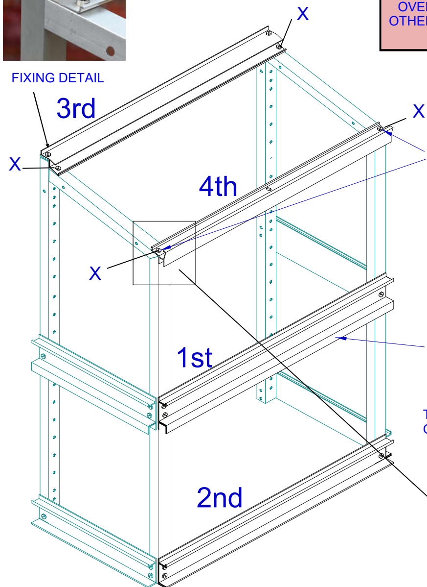
FIXING DETAIL
