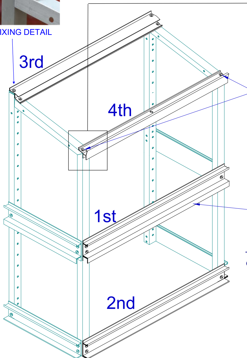
FIXING DETAIL
