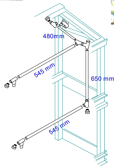
Double tee
