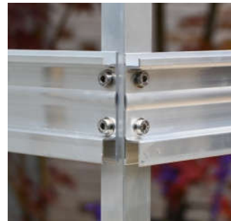
FIXING DETAIL
