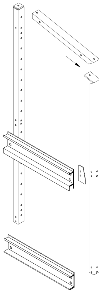
EXPLODED VIEW
