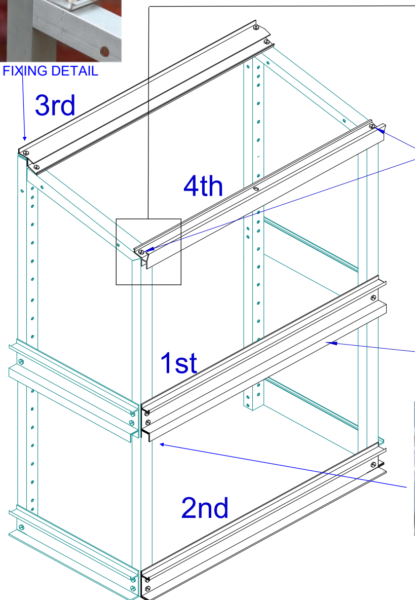
FIXING DETAIL
