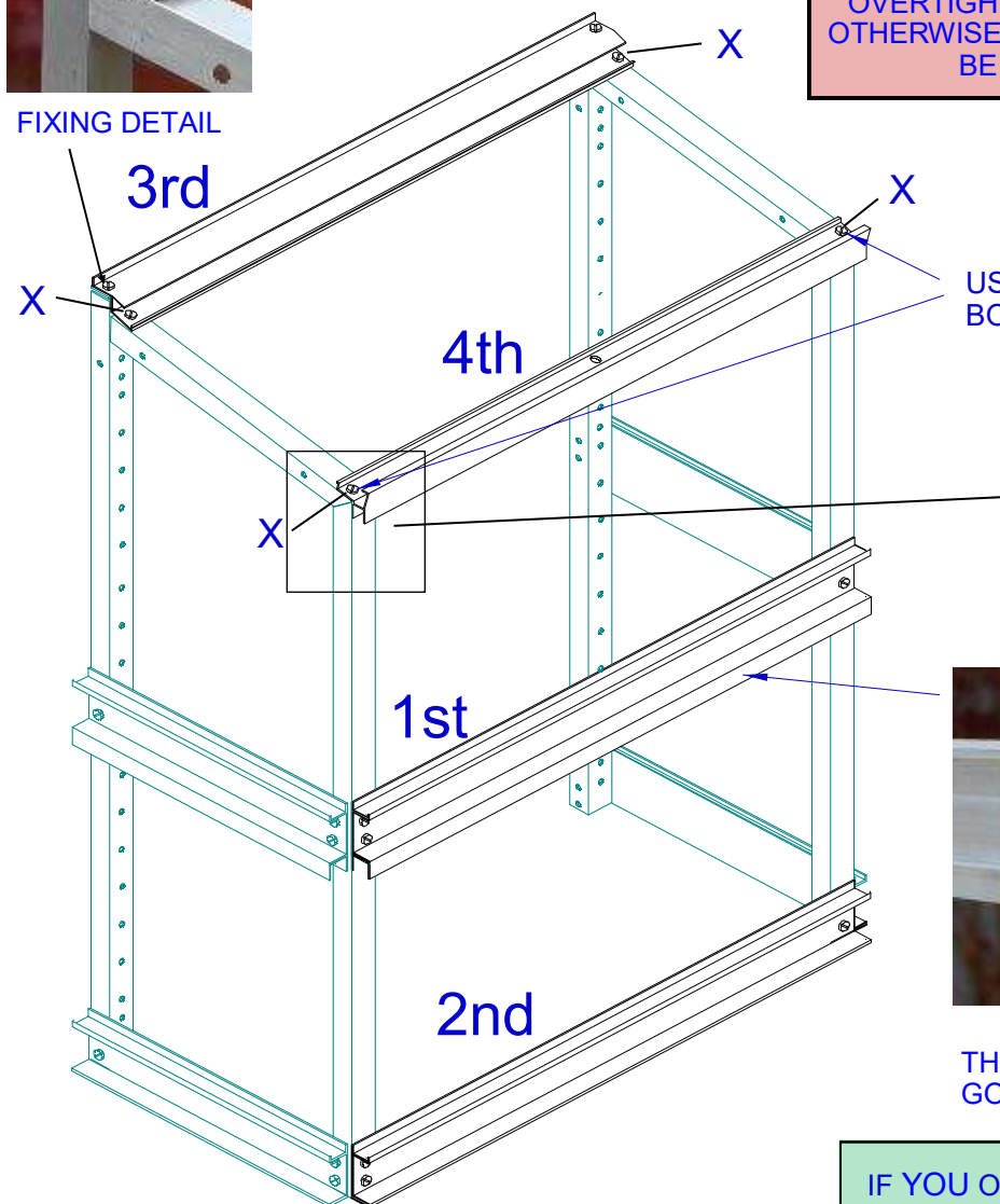
FIXING DETAIL
