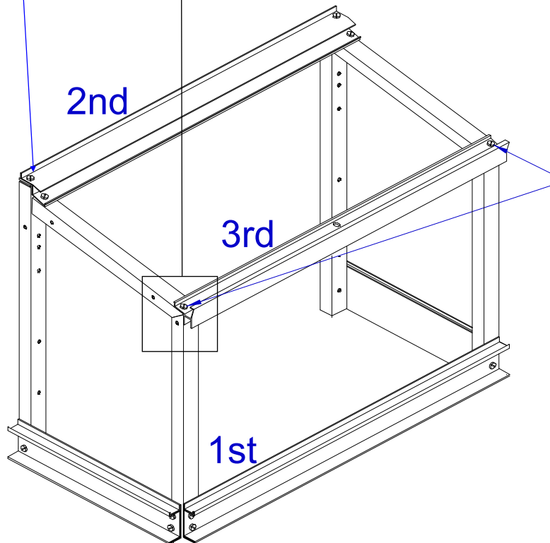
FIXING DETAIL
