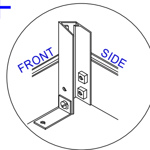
INSIDE VIEW OF FRONT LEG SHOWING FIXING
